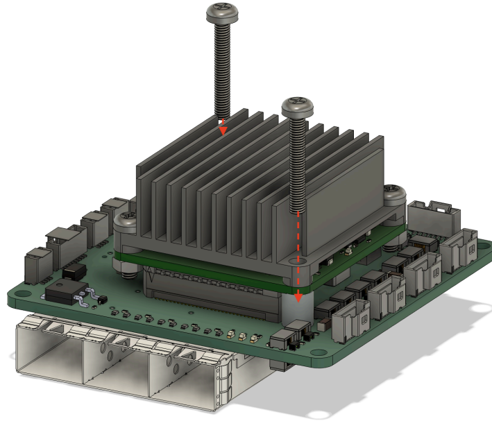
Figure 16. Mounting screws added to the remaining mount holes
