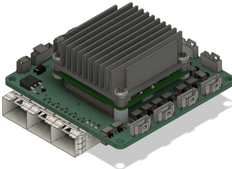
Figure 17. The final assembly
