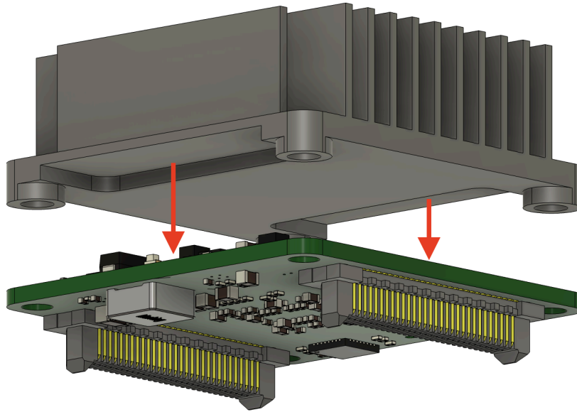
Figure 12. Aligning the heatsink to the UbiSwitch module. Removed material on the underside of the heatsink aligns with the taller components on two sides of UbiSwitch.
