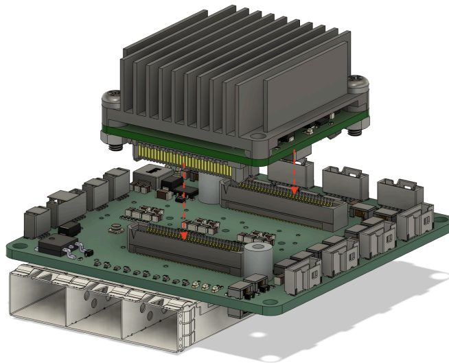
Figure 15. Mounting the UbiSwitch Module assembly onto the UbiSwitch BaseBoard
