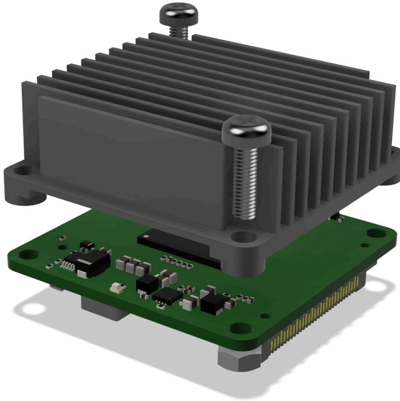
Figure 10. Illustration showing the UbiSwitch heatsink that is shipped with UbiSwitch
