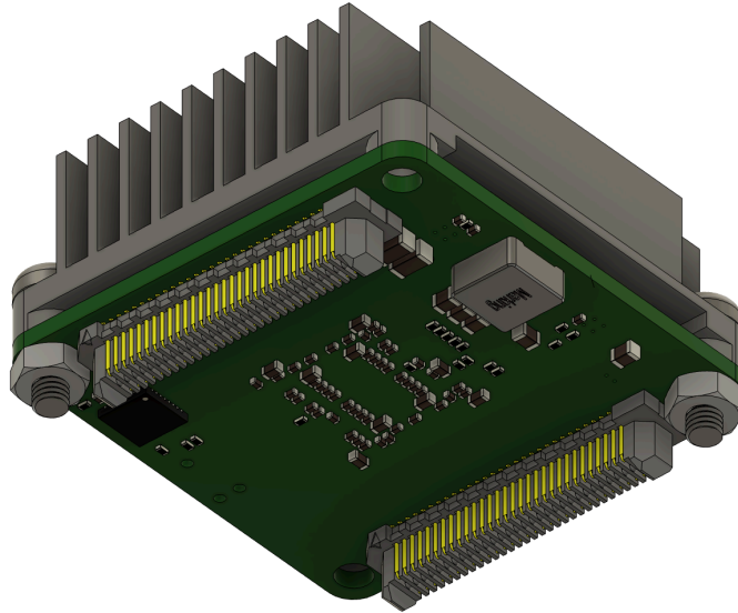
Figure 14. Adding the hex nuts to secure the heatsink
