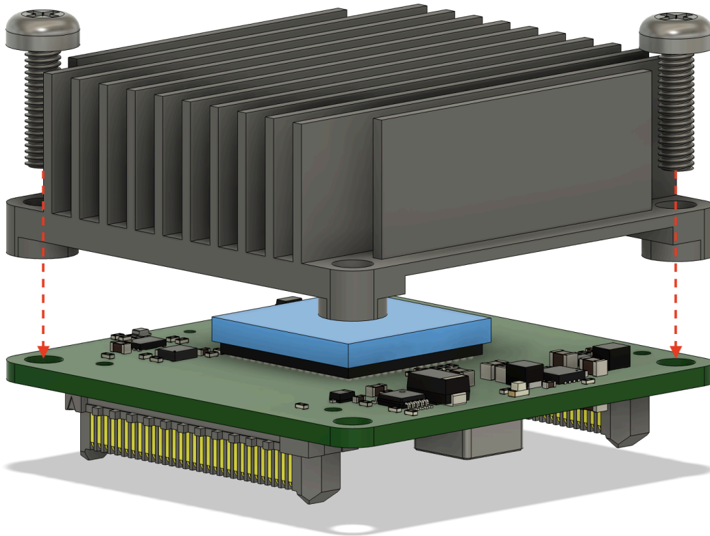
Figure 13. The machine screws for mounting the heatsink
