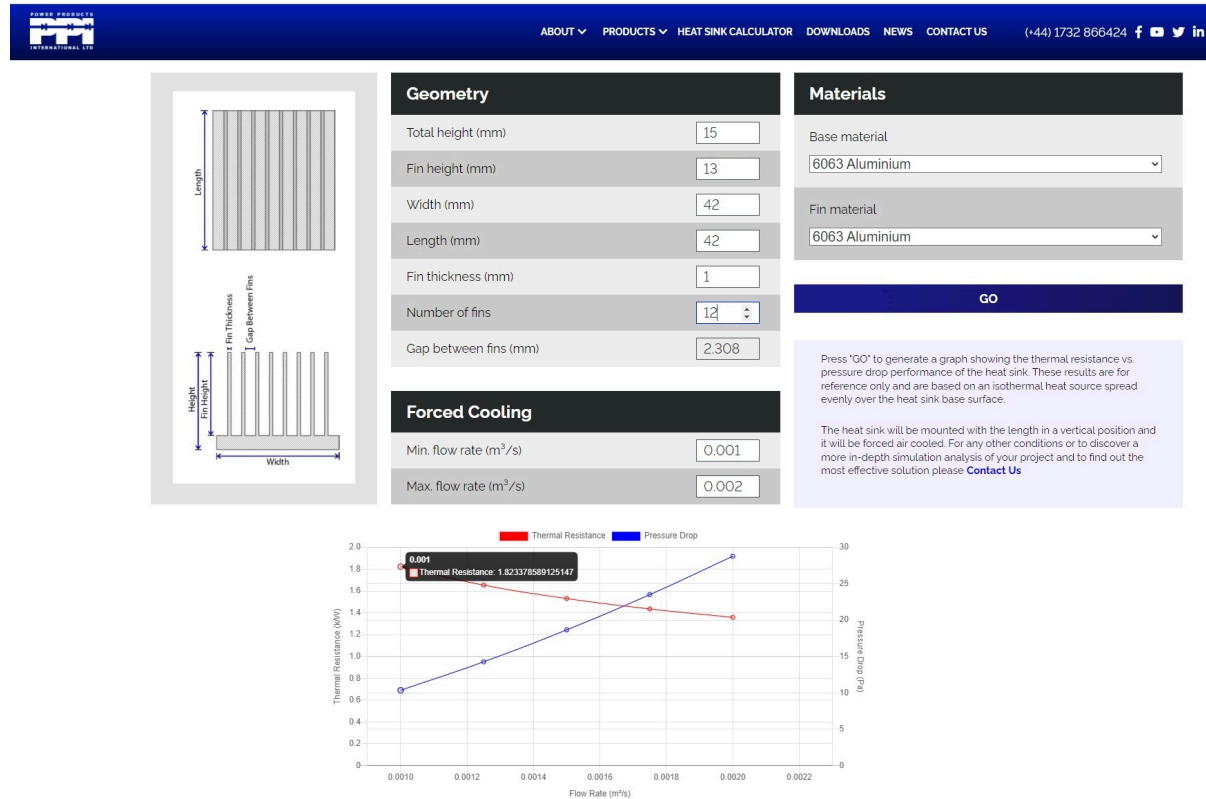
Figure 11. Thermal characteristics of the heatsink supplied with UbiSwitch
