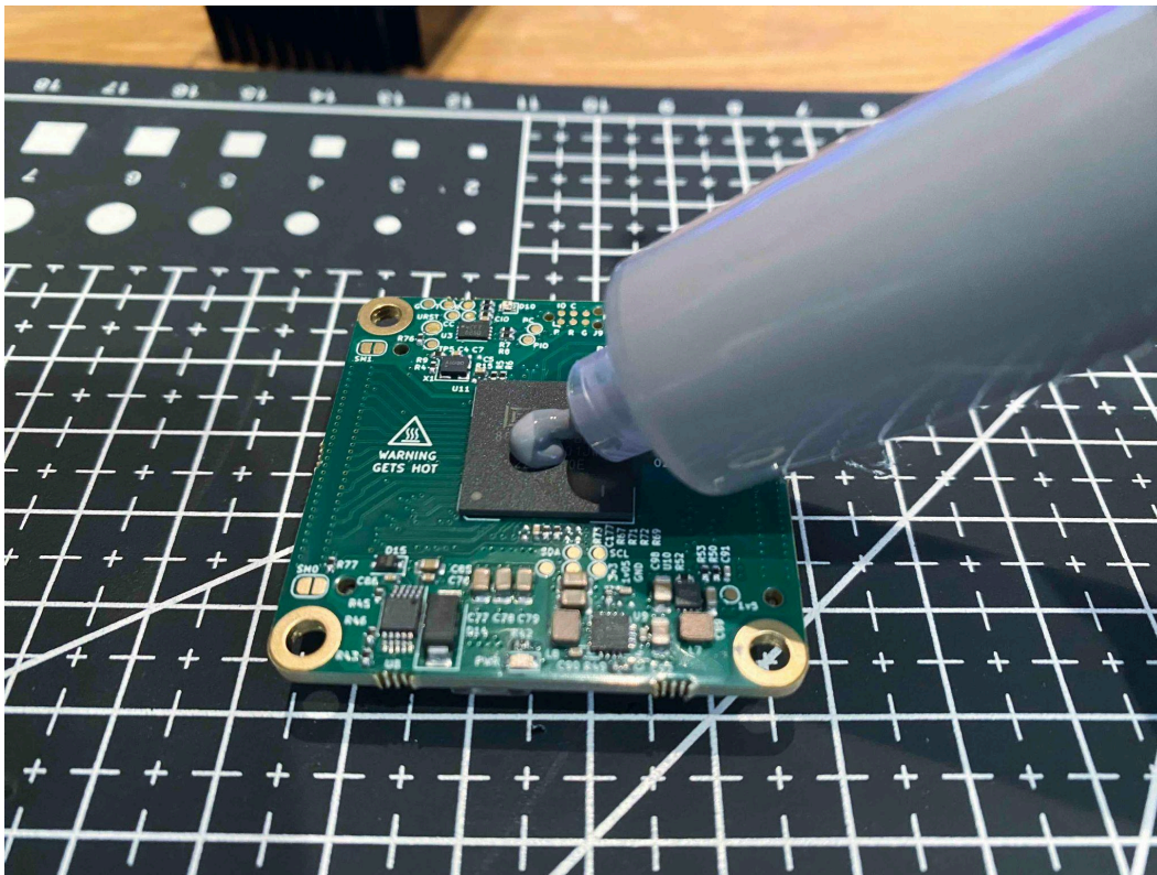
Figure 12. Applying thermal paste to UbiSwitch
