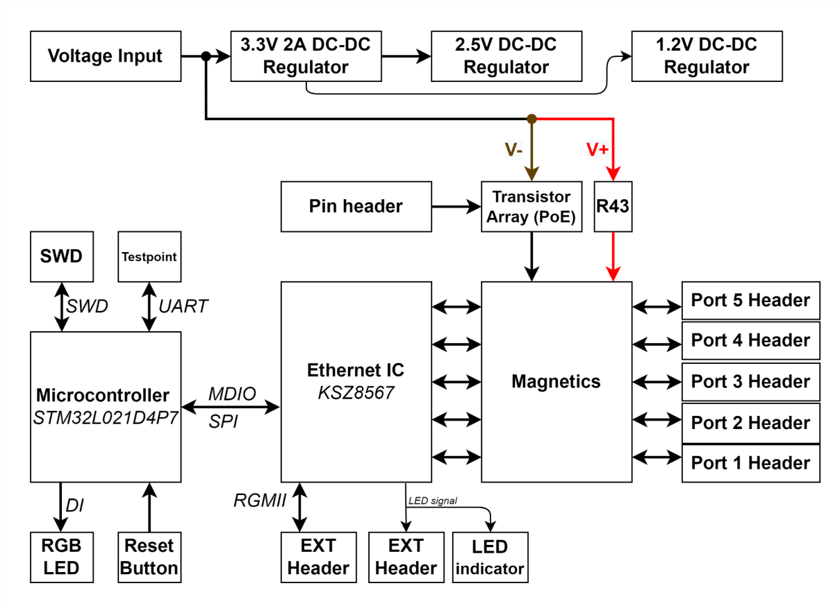
Figure 1: SwitchBlox Rugged Block Diagram
