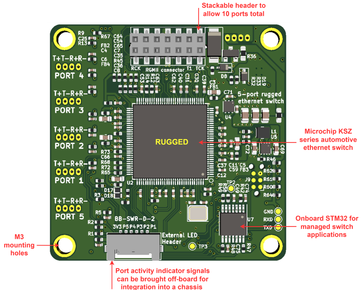
Figure 3: SwitchBlox Rugged Board Map (back)
