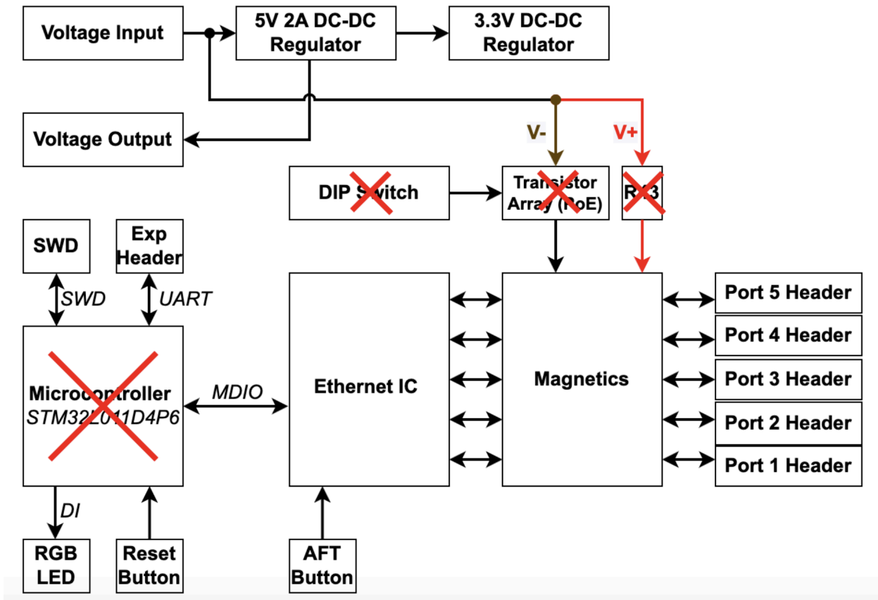
Figure 1: SwitchBlox Block Diagram
