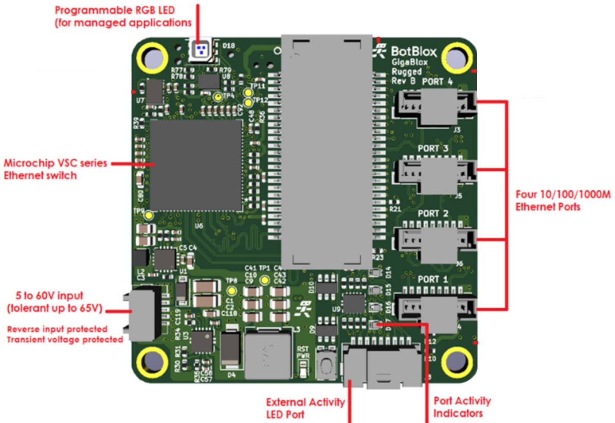
Figure 2: GigaBlox Rugged Board Map (front)
