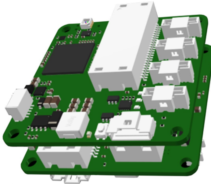
Figure 9: Stackable board
