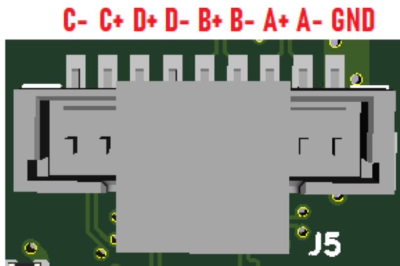
Figure 6: Ethernet port pinout
