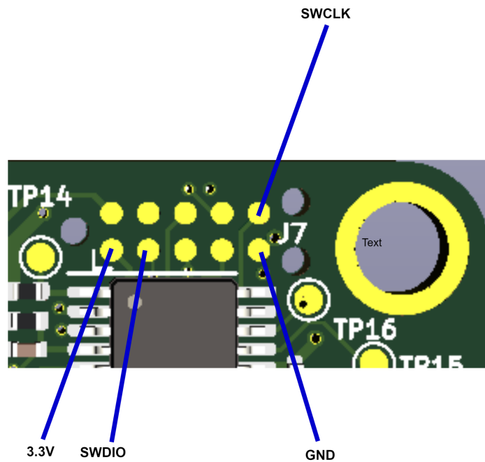
Figure 11: SWD programming header pinout
