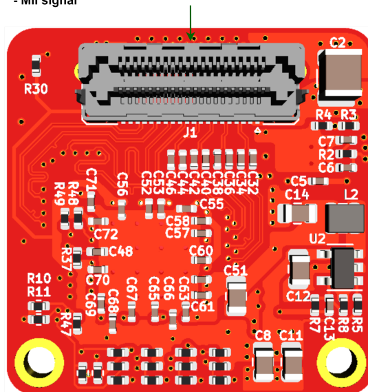
Figure 3: GigaBlox Nano Board Map (back)
