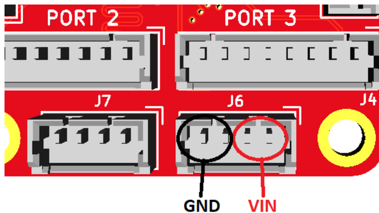
Figure 8: Mapping of power and ground onto PicoBlade connectors.
